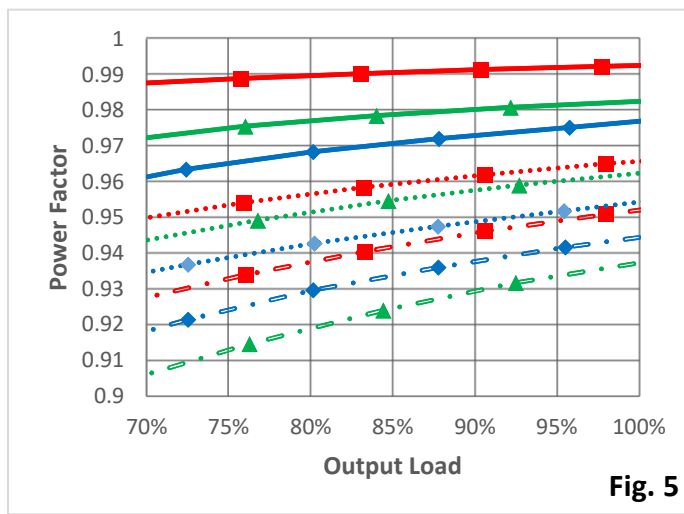
Power Factor vs. Load
