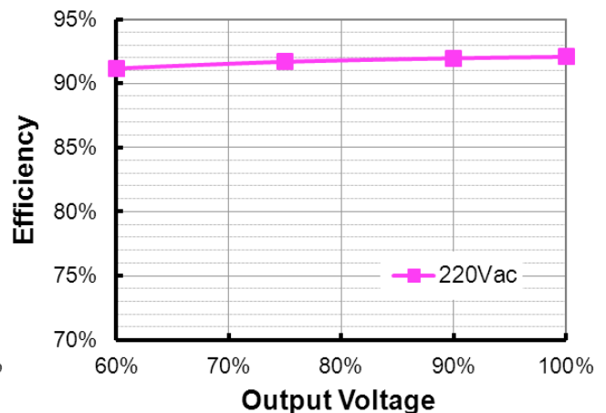
EDC-150S105SV-0004( I_o=860\text{mA} ) Efficiency vs. Output Voltage
