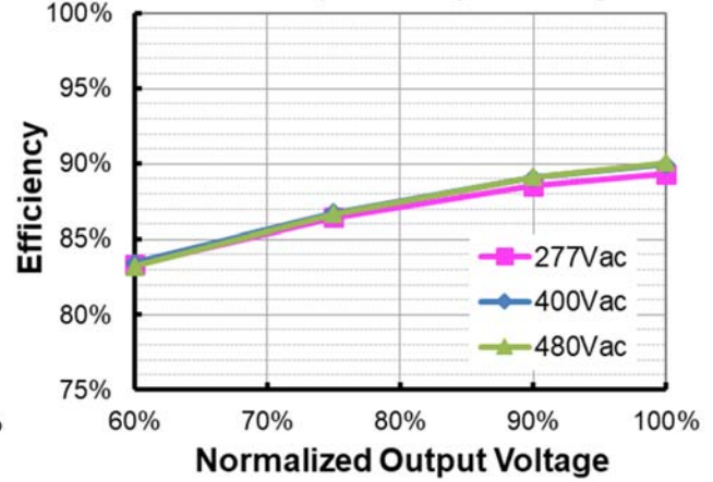
ESM-100S280Bx( I_o=2800\text{mA} ) Efficiency vs. Output Voltage
