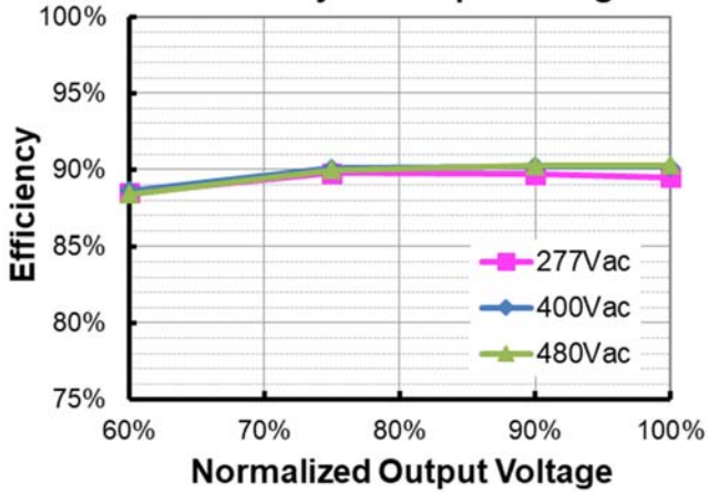
ESM-100S280Bx( I_o=1750\text{mA} ) Efficiency vs. Output Voltage
