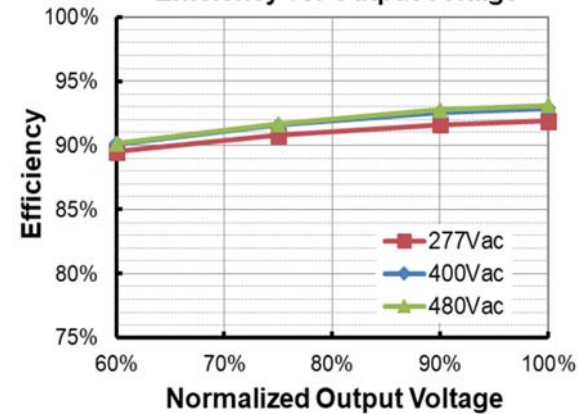
ESM-320S760Mx( I_o=7600mA ) Efficiency vs. Output Voltage
