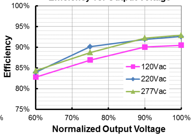
EUM-100S105Mx (I o =1050mA) Efficiency vs. Output Voltage
