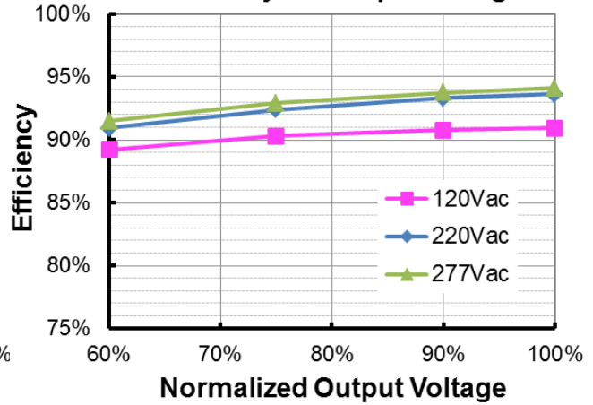
EUM-200S150Bx ( I_o=1500mA ) Efficiency vs. Output Voltage
