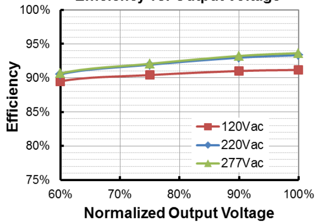
EUP-320S150SV (Io=1500mA) Efficiency vs. Output Voltage
