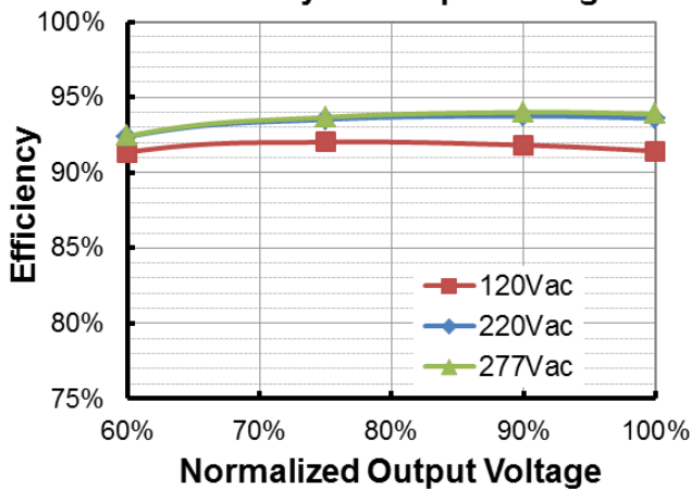
EUP-320S150SV (Io=1050mA) Efficiency vs. Output Voltage
