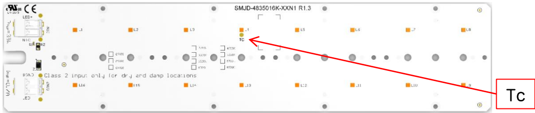
ILLUSTRATION 1: How to predict components temperature (4)
