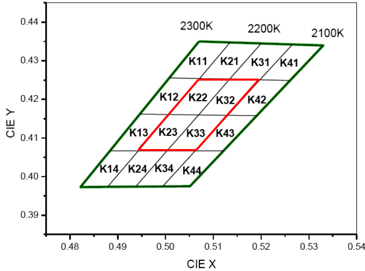
Fig 12. CIE Chromaticity Diagram
