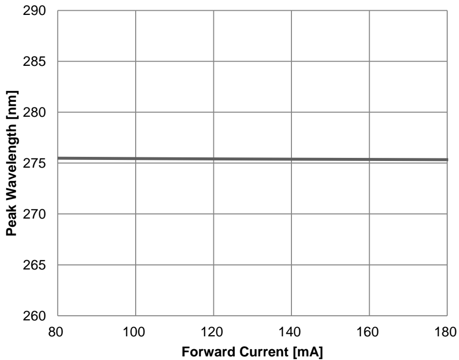
Fig 4. Forward Current vs. Peak Wavelength
