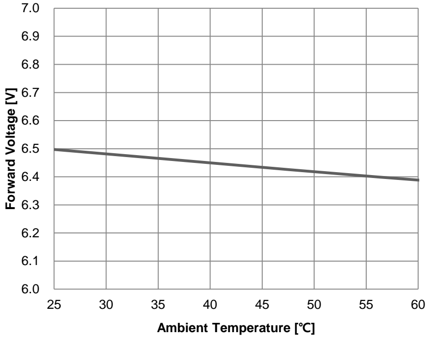
Fig 7. Ambient Temperature vs. Forward Voltage, I_F=120\text{mA}
