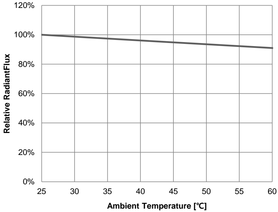
Fig 5. Ambient Temperature vs. Relative Radiant Flux, I_F=120mA
