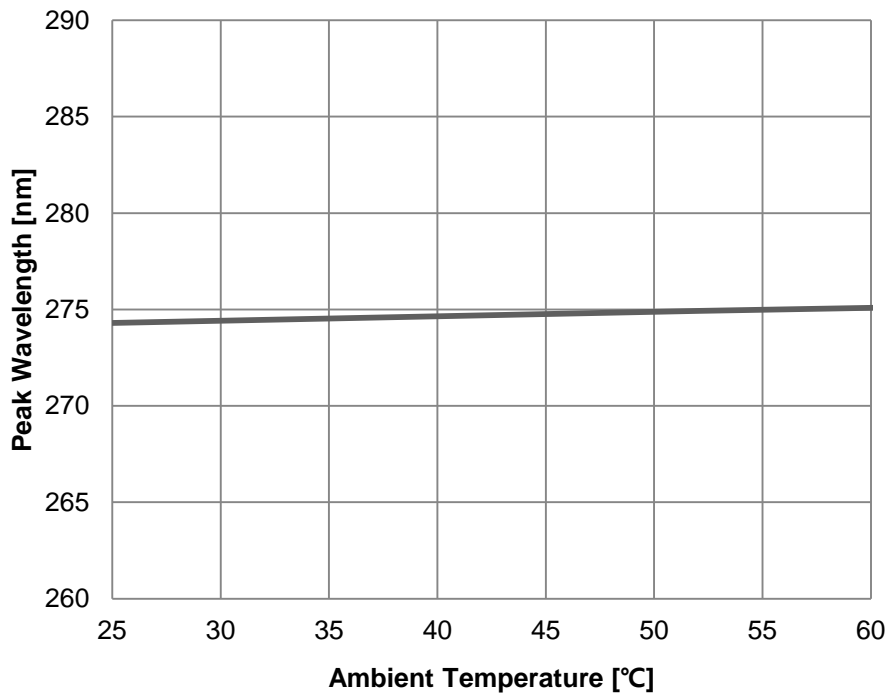
Fig 6. Ambient Temperature vs. Peak Wavelength, I_F=120mA
