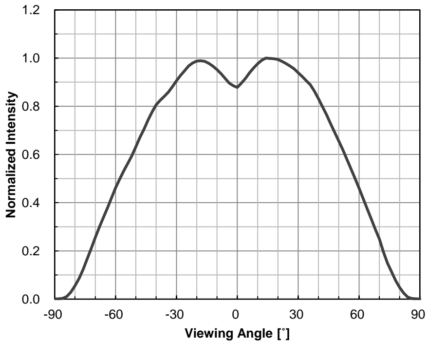
Fig 8. Typical Spatial Distribution, I_F=120\text{mA}
