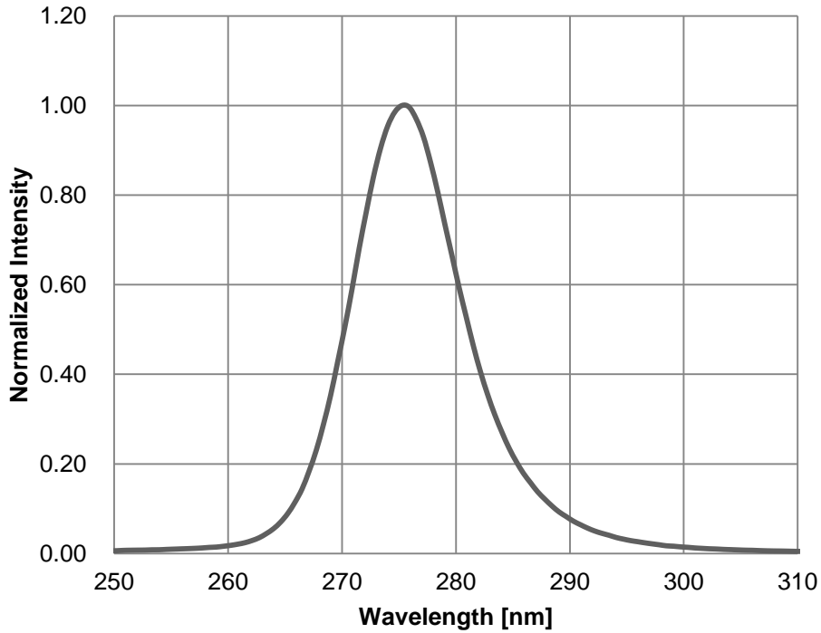
Fig 1. Spectrum, T_a=25^\circ\text{C} , I_F=120\text{mA}
