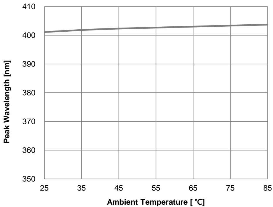
Fig 6. Ambient Temperature vs. Peak Wavelength, I_F=180mA
