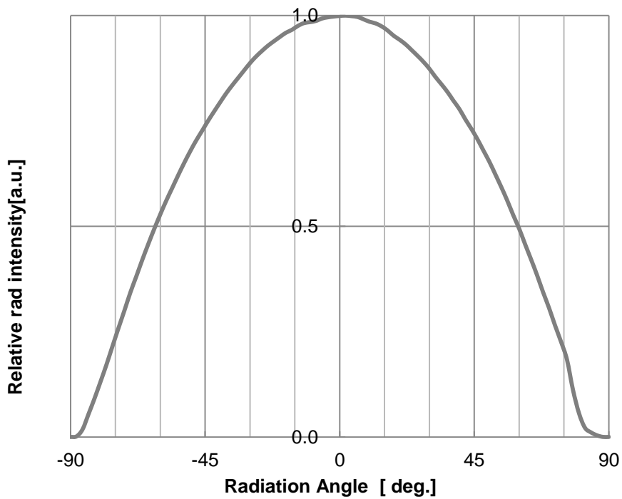
Fig 8. Typical Spatial Distribution, I_F=180\text{mA}
