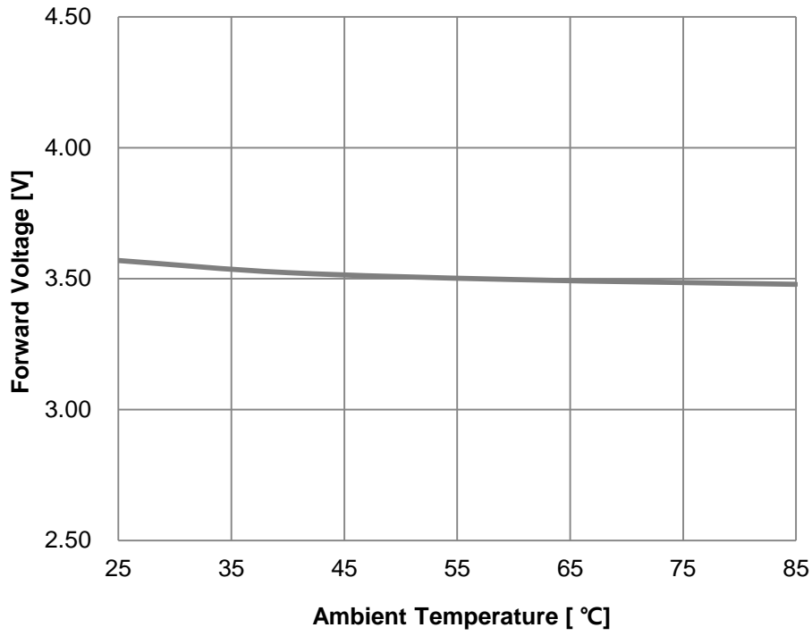
Fig 7. Ambient Temperature vs. Forward Voltage, I_F=180\text{mA}
