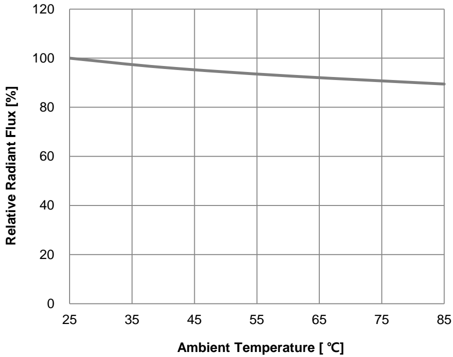
Fig 5. Ambient Temperature vs. Relative Radiant Flux, I_F=180mA
