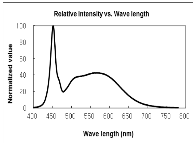
CCT : 6500K (80 CRI)
