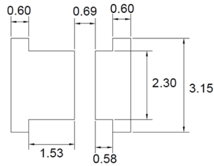
[RECOMMENDED PCB SOLDER PAD]
