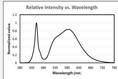
CCT : 4000K (70 CRI)
