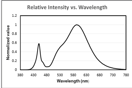
CCT : 2700K (70 CRI)
