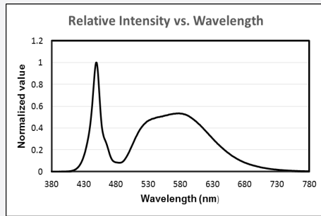
CCT : 5000K (70 CRI)
