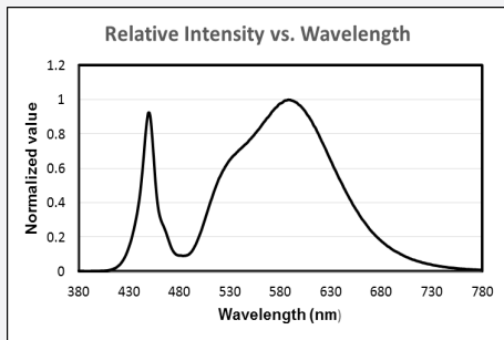
CCT : 3500K (70 CRI)
