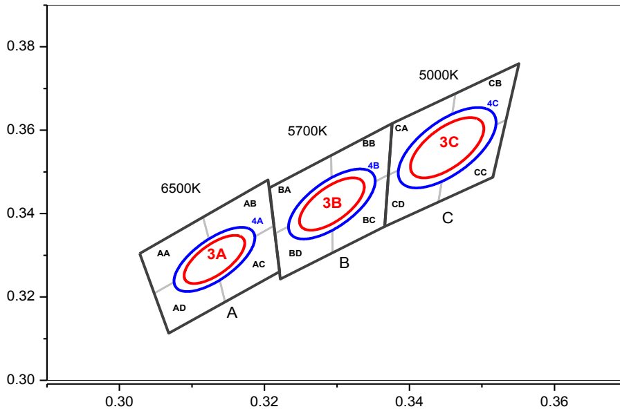
CIE Chromaticity Diagram T_j=25^{\circ}\text{C} , I_F=150\text{mA}
