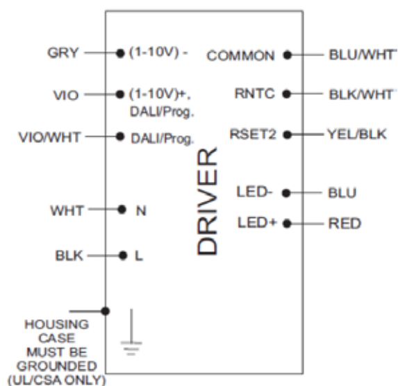
Wire Diagram
