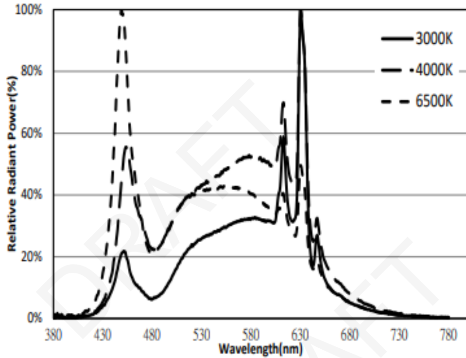
Figure 10: Typical Color Spectra, 90 CRI
