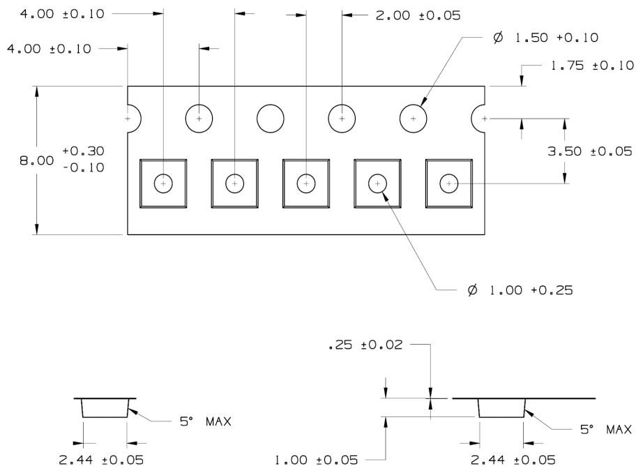
Figure 13. Pocket tape dimensions for LUXEON Versat 2020 CW 150
