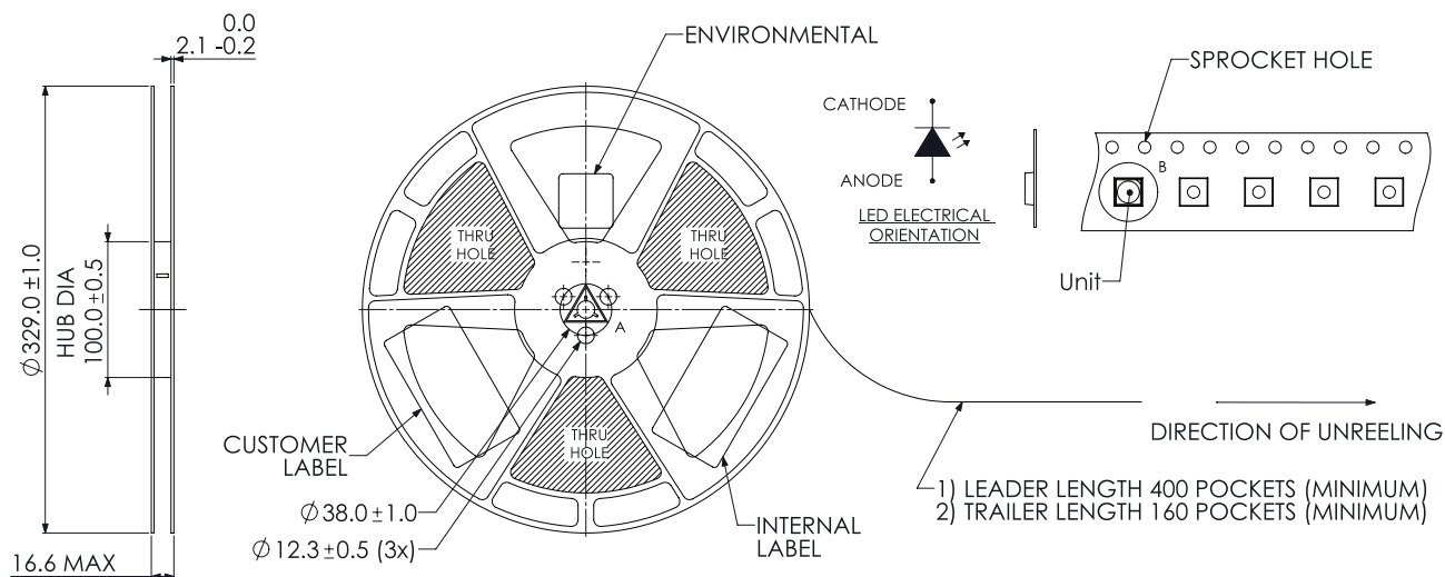
Figure 14. Reel dimensions for LUXEON Versat 2020 CW 150
