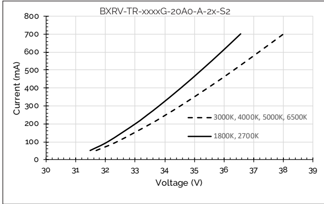
Figure 5: Forward Voltage vs. Forward Current, T_c=25^\circ\text{C}
